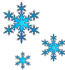
snowflakes
